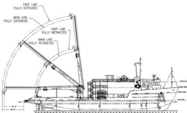
Outboard Profile
