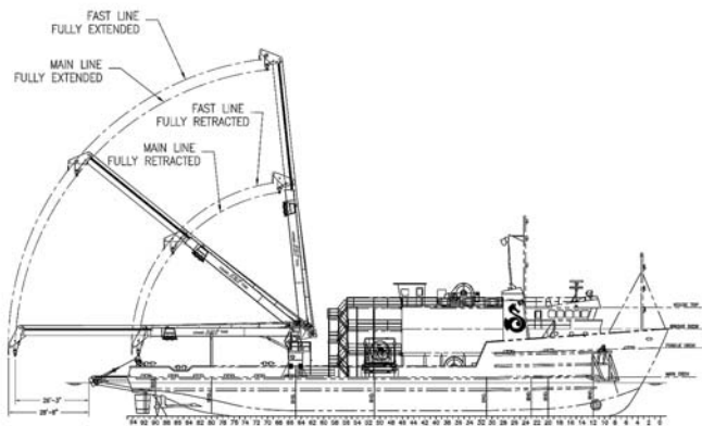
Outboard Profile
